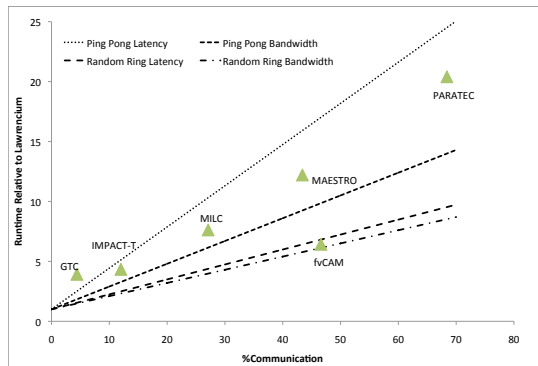
Fig. 3. Correlation between the runtime of each application on EC2 and the amount of time an application spends communicating.
